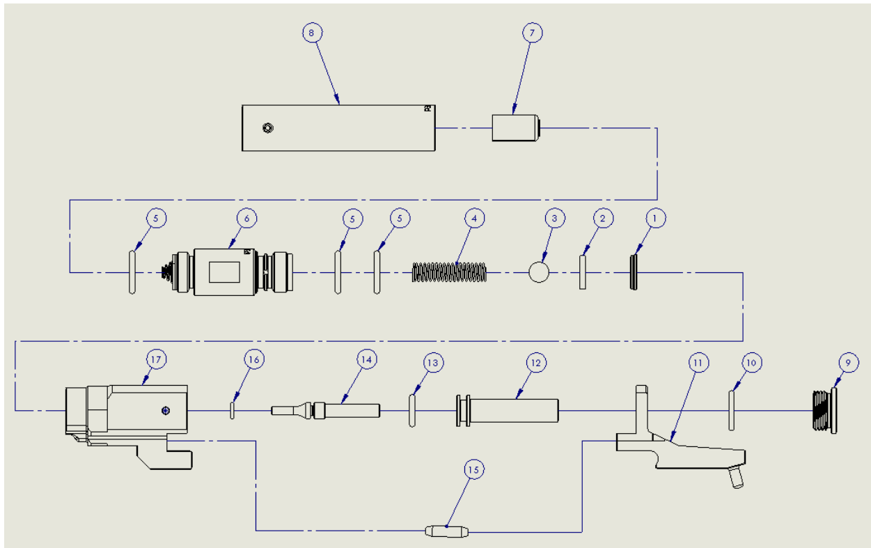
Figure 1: Barrel Assembly
